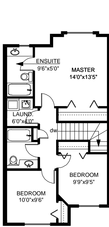
UPPER FLOOR 691 SQ.FT
