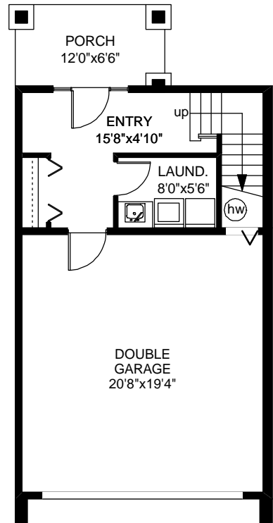
LOWER FLOOR 227 SQ.FT
