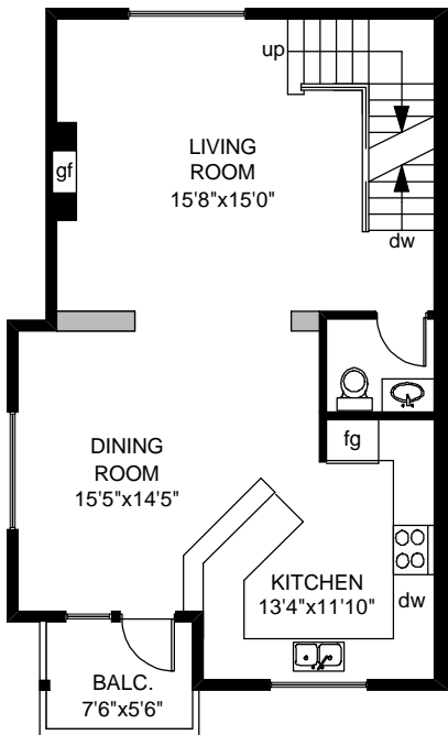
MAIN FLOOR 692 SQ.FT
